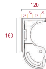
supporto universale universal fixing bracket
